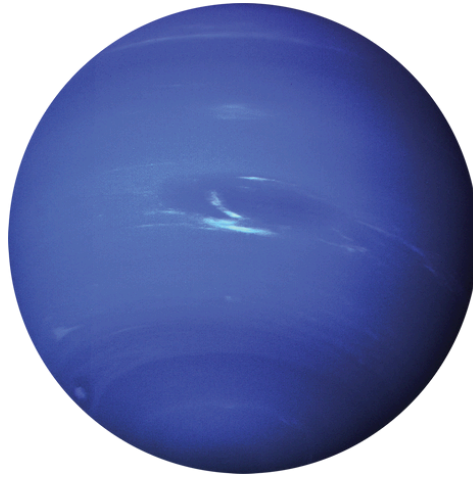
Neptune
