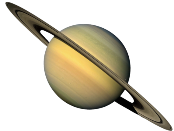
Saturn
